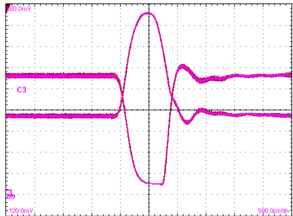
Figure 5. DC-coupled laser driver output with the HDTV-SDI test pattern, middle of pathological region (standard APC loop).
