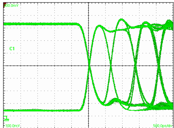
Figure 10. MAX3656 optical eye with the HDTV-SDI test pattern, end of pathological region.
