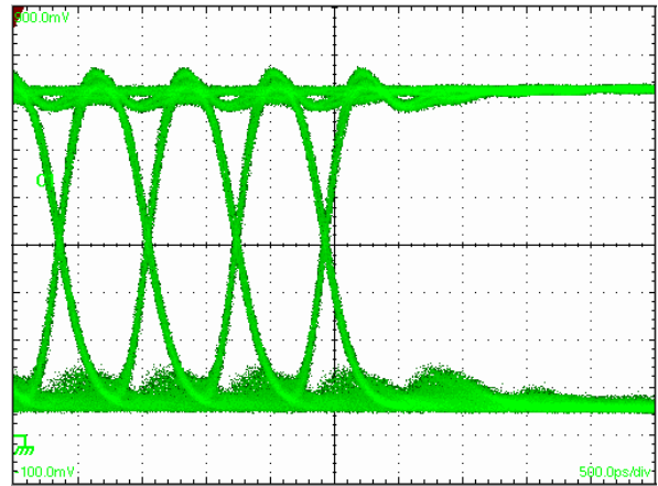
Figure 8. MAX3656 optical eye with the HDTV-SDI test pattern beginning of pathological region.
