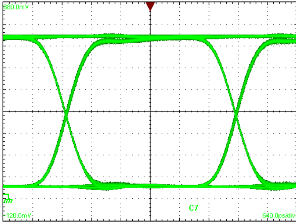
Figure 11. MAX3656 optical eye with 2^{31}-1 PRBS at 270Mbps.
