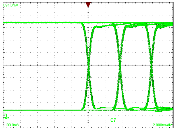
Figure 14. MAX3656 optical eye with the SDTV-SDI test pattern, end of pathological region.
