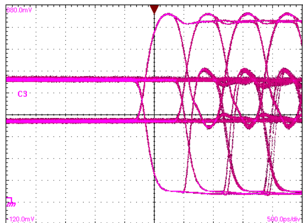
Figure 6. DC-coupled laser driver output with the HDTV-SDI test pattern, exiting pathological region (standard APC loop).
