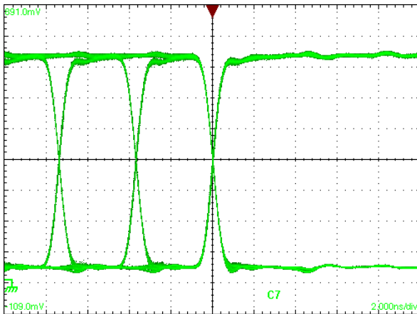
Figure 12. MAX3656 optical eye with the SDTV-SDI test pattern, beginning of pathological region.
