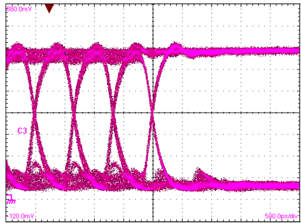
Figure 4. DC-coupled laser driver output with the HDTV-SDI test pattern, entering the pathological region (standard APC loop).
