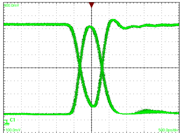
Figure 9. MAX3656 optical eye with the HDTV-SDI test pattern, middle of pathological region.
