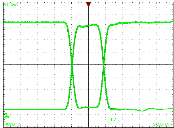
Figure 13. MAX3656 optical eye with the SDTV-SDI test pattern, middle of pathological region.
