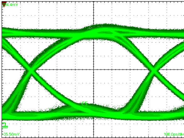
Figure 7. MAX3656 optical eye with a 2^{31}-1 PRBS operating at 1.485Gbps.
