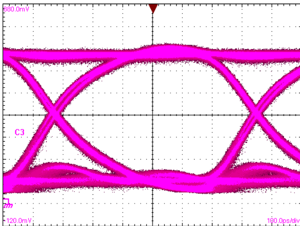
Figure 3. DC-coupled laser driver output with 2^{31}-1 PRBS operating at 1.485Gbps (standard APC loop).
